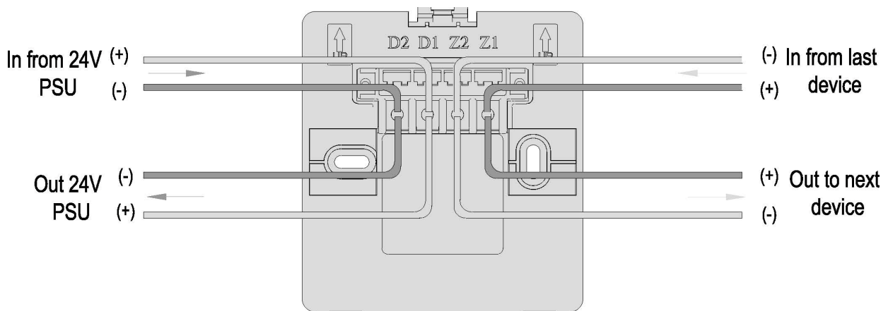
Figure 3: Wiring Details
